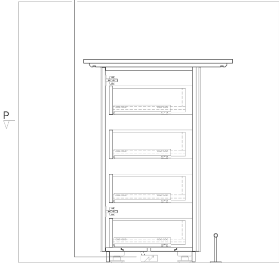
SECTION S1-S1' / SCALE 1:20
