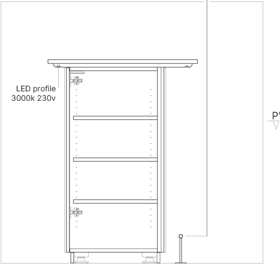
SECTION S2-S2' / SCALE 1:20
