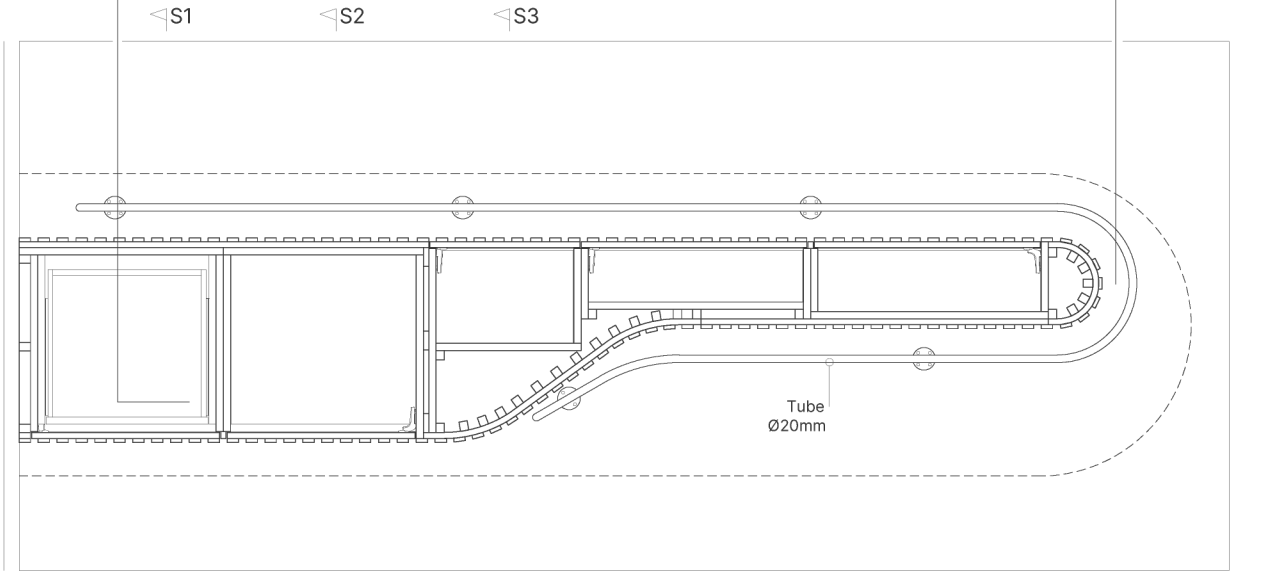
PLAN P-P' / SCALE 1:20
